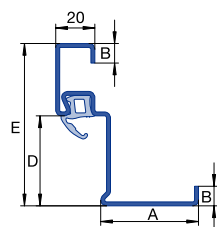
Eckzarge
